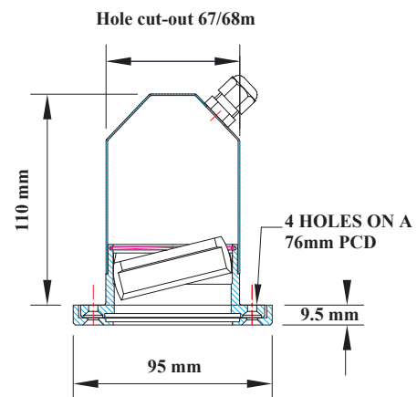
Dimension for flush deckhead fitting
