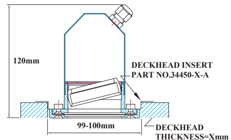
Dimension for flush deckhead fitting
