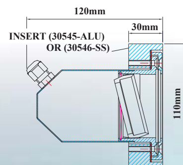
Dimension for flush weld-in fitting
